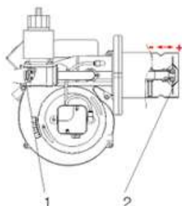
[Figura 2G-F. MAXI 20S]
