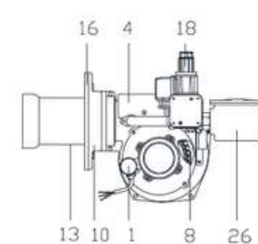
[Figura 3E-B. MAXI 8, 10, 16]
